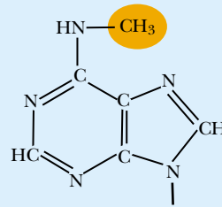
N 6 METHYLADENOSINE
