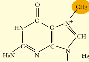
7-METHYLGUANOSINE
