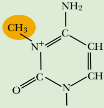
3-METHYLCYTIDINE
