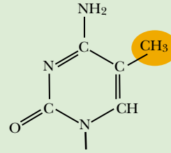
5-METHYLCYTIDINE
