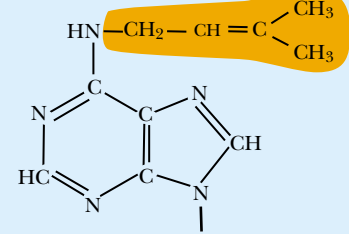
N 6 ISOPENTENYLADENOSINE
