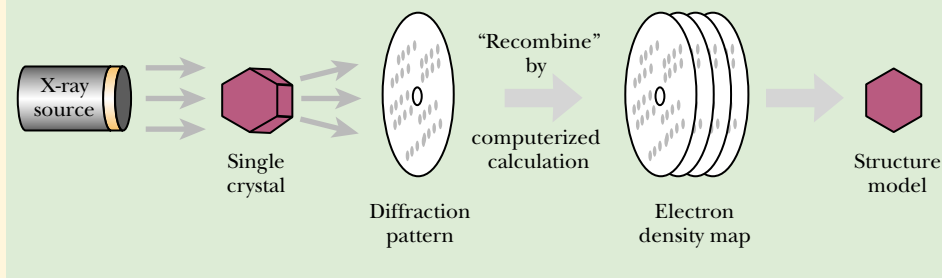
FIGURE 7.20 X-ray Crystallography
