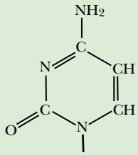
CYTIDINE
