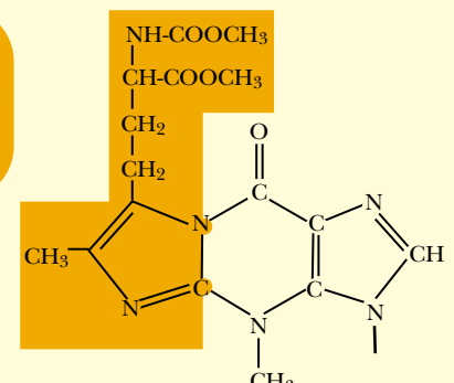
WYOSINE (Y)
